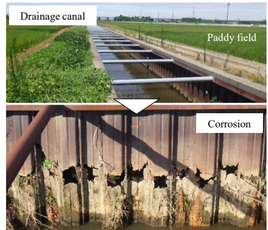
Severe corrosion of steel sheet pile walls.
