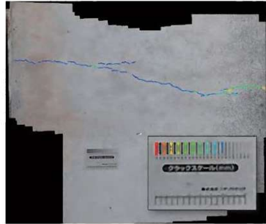
Detection and classification of cracks on concrete structures using video recorded with mobile devices.
