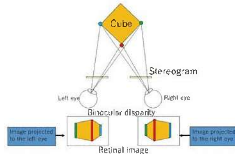
Schematic diagram of the difference in retinal images when observing a cube
