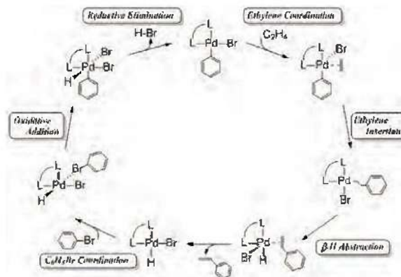
New Heck catalytic cycle with Pd (II) complex
