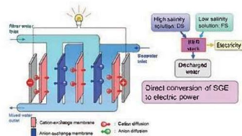
Reverse electrodialysis system (RED) for energy production
