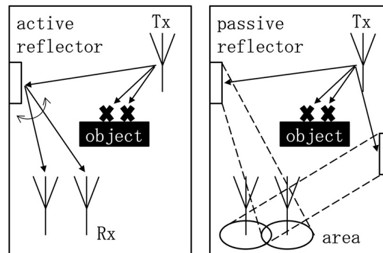
Active and passive reflectors
