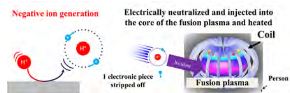
Overview of Negative Ion Generation and Its Applications in Fusion Reactors
