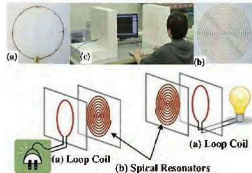
Wireless Power Transfer System
