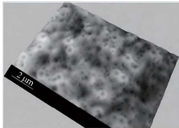
Direct observation of nanoscopic emission distribution of InGaIn semiconductor alloy by Cathodoluminescence mapping
